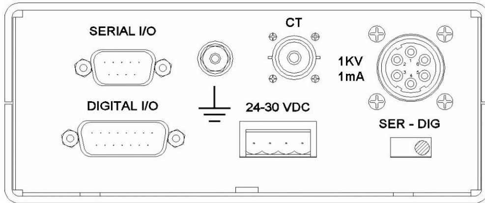
Figure 2.1 - EPS300 Front Panel
