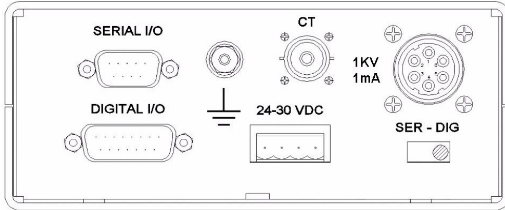
Figure 3.1 - EPS300 Front Panel
