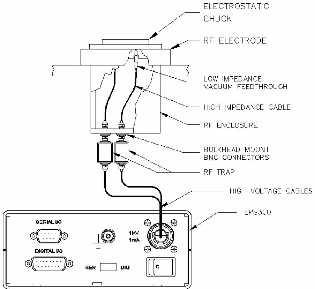
Figure 2.3 – EPS300 Typical Installation
