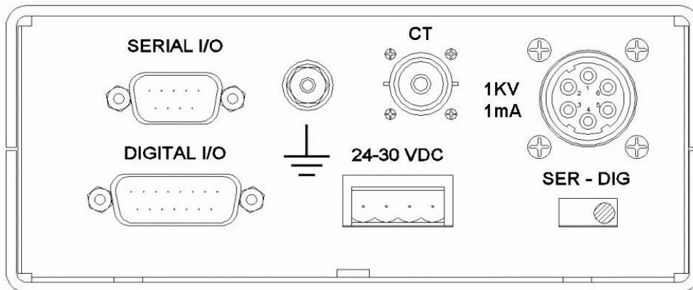
Figure 2.2 - EPS300 Front Panel
